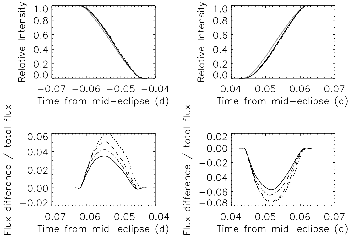
FIG. 2.— Upper left : Ingress portion of the secondary eclipse light curves of HD 209458b, assuming a uniform flux distribution (solid gray line) and the CS05 model for the spatial flux variation (dashed lines overlying each other). Lower left : The relative differences in the curves resulting from the CS05 model to the prediction of the uniform flux distribution, for the four IRAC band passes ( 3.6\ \mu\text{m} , dotted lines; 4.5\ \mu\text{m} , dashed lines; 5.8\ \mu\text{m} , dash-dotted lines; and 8.0\ \mu\text{m} , solid lines). The right panels depict these curves and their differences at egress.
