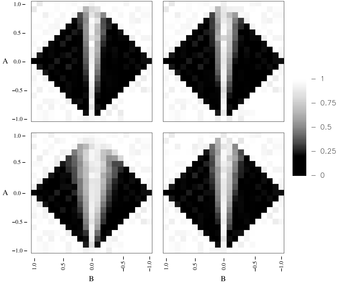
FIG. 4.—Diamonds representing P_0 values (§ 4.2) over the (A, B) parameter space of the sinusoidal planetary model as determined by Monte Carlo simulations of IRAC observations (upper left, 3.6 \mu\text{m} ; upper right, 4.5 \mu\text{m} ; lower left, 5.8 \mu\text{m} ; and lower right, 8.0 \mu\text{m} ). If a value of t_{\text{offs}} = 0 were to be observed for the HD 209458 system, models corresponding to the dark squares could be excluded with high confidence, whereas models corresponding to the lighter squares could not. The A parameter controls the latitudinal flux contrast while the B parameter controls the longitudinal flux contrast. Although the dominant sensitivity is to longitudinal contrast, note the effect of the non-equatorial orbit, which permits a modest sensitivity to latitudinal flux variations. Models with |A| + |B| > 1 were not considered because they would yield areas of the planet presenting a negative flux.
