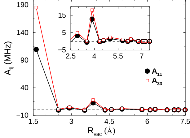
FIG. 7: Variation of the principal values of the hyperfine tensor A_{11} and A_{33} as a function of the distance from the vacant site ( R_{vac} ) for the set of 3 symmetrically equivalent C atoms (3C). In the inset we show changes farther from the vacant site on a finer scale. The variation for the set of 6 symmetrically equivalent C atoms follows closely the one shown for 3C.
