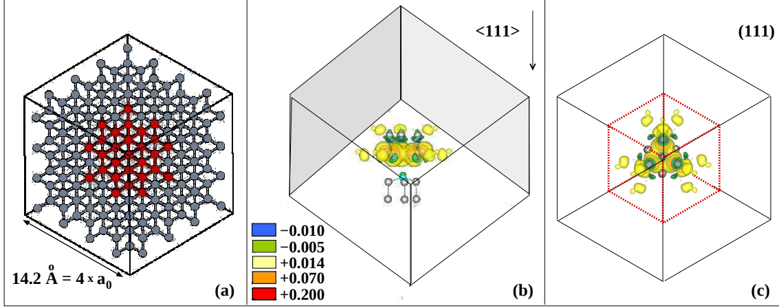
FIG. 6: (Color online) (a) The 512-atom cubic supercell with all C atoms shown (atoms within a 64-atom supercell are shown in red). The supercell size in Å and in units of the conventional cubic cell lattice constant, a_0 , is indicated on the side of the cube. (b) Perspective view of the calculated spin density isosurfaces in the M_S=1 state. Only atoms up to the second nearest neighbor of the vacant site are shown. (c) View along the (111) direction indicating the C_{3v} symmetry of the spin density, which is given in colored contours. The black lines denote the size of the 512-atom supercell, while the red dotted ones show the boundaries of the 64-atom supercell.
