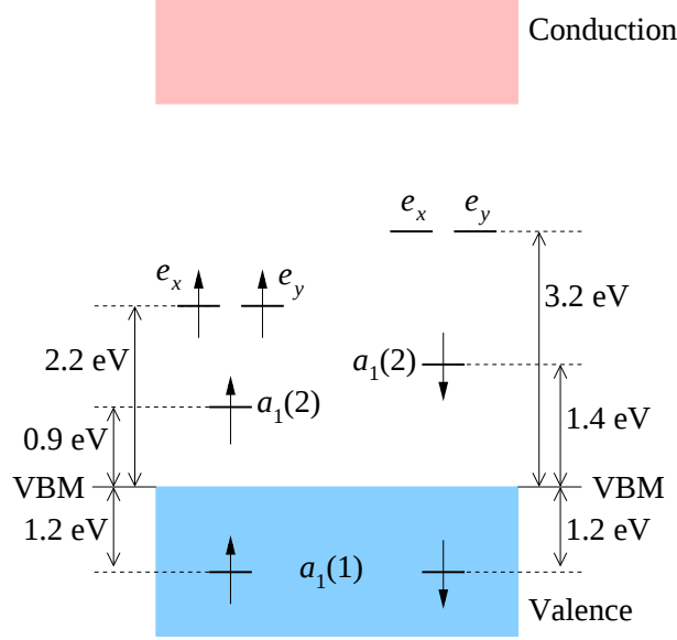
FIG. 2: (Color online) The calculated spin-resolved single-electron levels with respect to the valence band maximum (VBM) in the ground state of the NV defect. Valence and conduction bands of the host crystal are shown as blue and pink shaded regions, respectively. The levels are labeled as in Eq. (1) and their occupation is given for a negatively charged defect (a total of 6 electrons).
