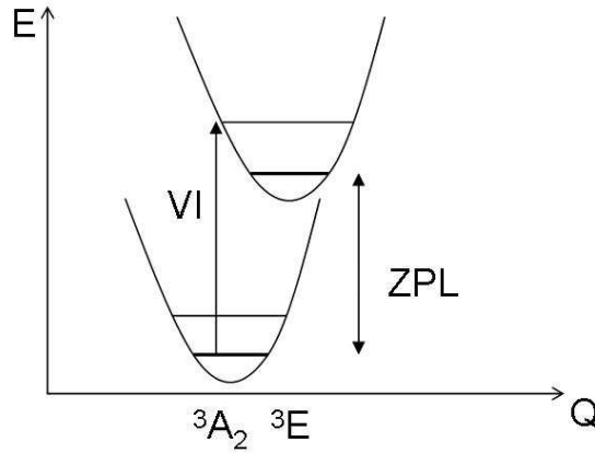
FIG. 5: Energetics of photoluminescence absorption: VI is the vertical ionization energy, ZPL is the zero-phonon line transition, E is the total energy and Q the configuration coordinate.
