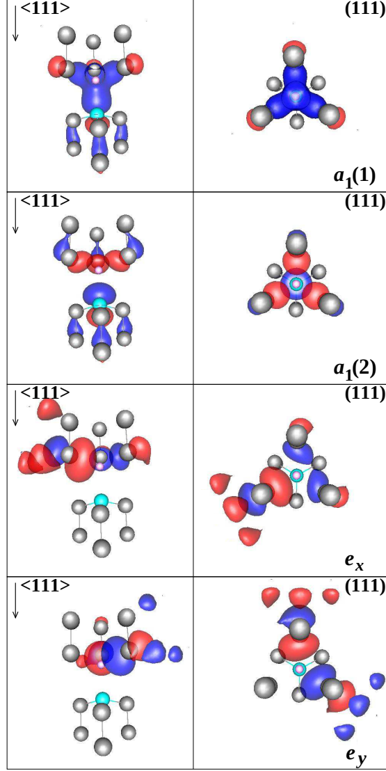
FIG. 3: (Color online) Isosurfaces of the calculated wavefunctions of the a_1(1) , a_1(2) , e_x , e_y defect states, shown in side (left) and top (right) views relative to the \langle 111 \rangle axis. Blue (red) isosurfaces correspond to negative (positive) values of the wavefunction. The small pink circle represents the position of the vacant site, while the grey and cyan balls show the C and N atoms, respectively. We show the atoms up to the second neighbor from the vacant site.
