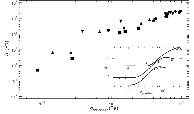
FIG. 3. Elasticity of shear thickened gels as a function of the pre-shear stress, using cone-plate geometry. ■: 3%, ▲: 4%, ●: 5%, ◆: 6%, ▼: 8%. Inset: Data obtained spanning low and high stresses using a double-wall Couette cell. +: 2%, □: 3%, ○: 5%.
