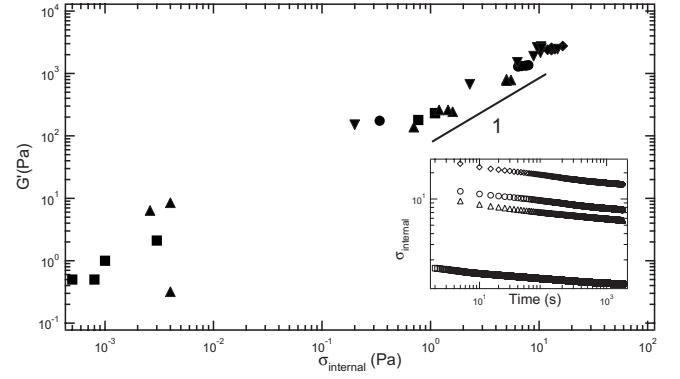
FIG. 5. Shear modulus scales linearly with residual stresses resulting from the quench into the gel state on cessation of flow. ■: 3%, ▲: 4%, ●: 5%, ◆: 6%, ▼: 8%. The solid line is a visual guide with a slope of 1. Inset: Time dependence of internal stress, with open symbols for clarity.
