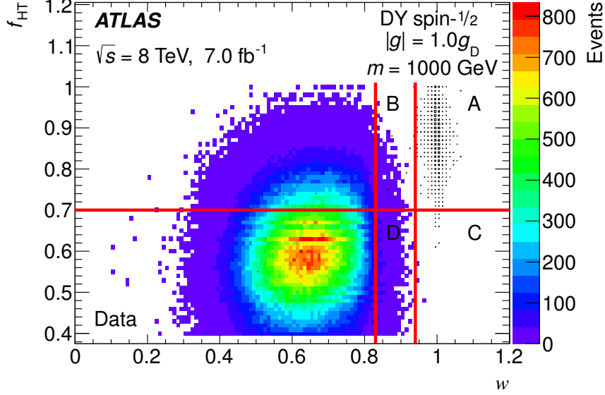
Figure 4: Candidates seen in data (color scale) and in a representative simulated signal sample (black squares) in the f_{\text{HT}} versus w plane, at the last stage of the event selection (prior to the requirements on these two variables). The number of background events in the signal region (A) is estimated using the left and bottom bands (B, D, and C) as control regions, as described in the text.
