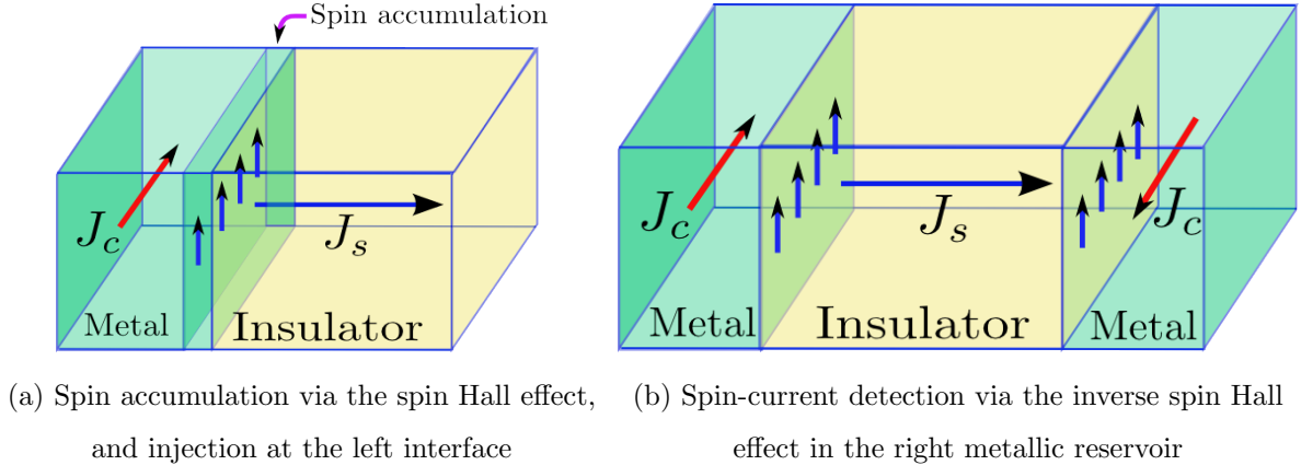
FIG. 1: Geometry for generation and detection of spin-current
