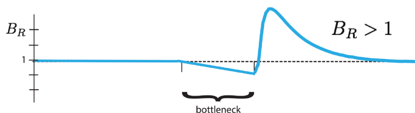
Fig 1. Response of the B_R statistic for additive and recessive variation. A schematic representation of two populations is presented above (A). Initially a single population prior to the bottleneck event, the populations split and have distinct demographic profiles. The equilibrium population maintains a constant size for easy comparison to the founded population. The latter drastically reduces its population size to N_B for a short time T_B during the founder's event. Our statistical comparison between populations B_R = \frac{\langle x \rangle_{eq}}{\langle x \rangle_{founded}} is represented here for cases of purely additive (B) and purely recessive (C) variation. The statistic B_R > 1 for recessive variation (dominance coefficient h = 0 ) and B_R < 1 for additive variation ( h = 1/2 ), providing a simple indicator for the primary mode of selection of polymorphic alleles in the populations.
