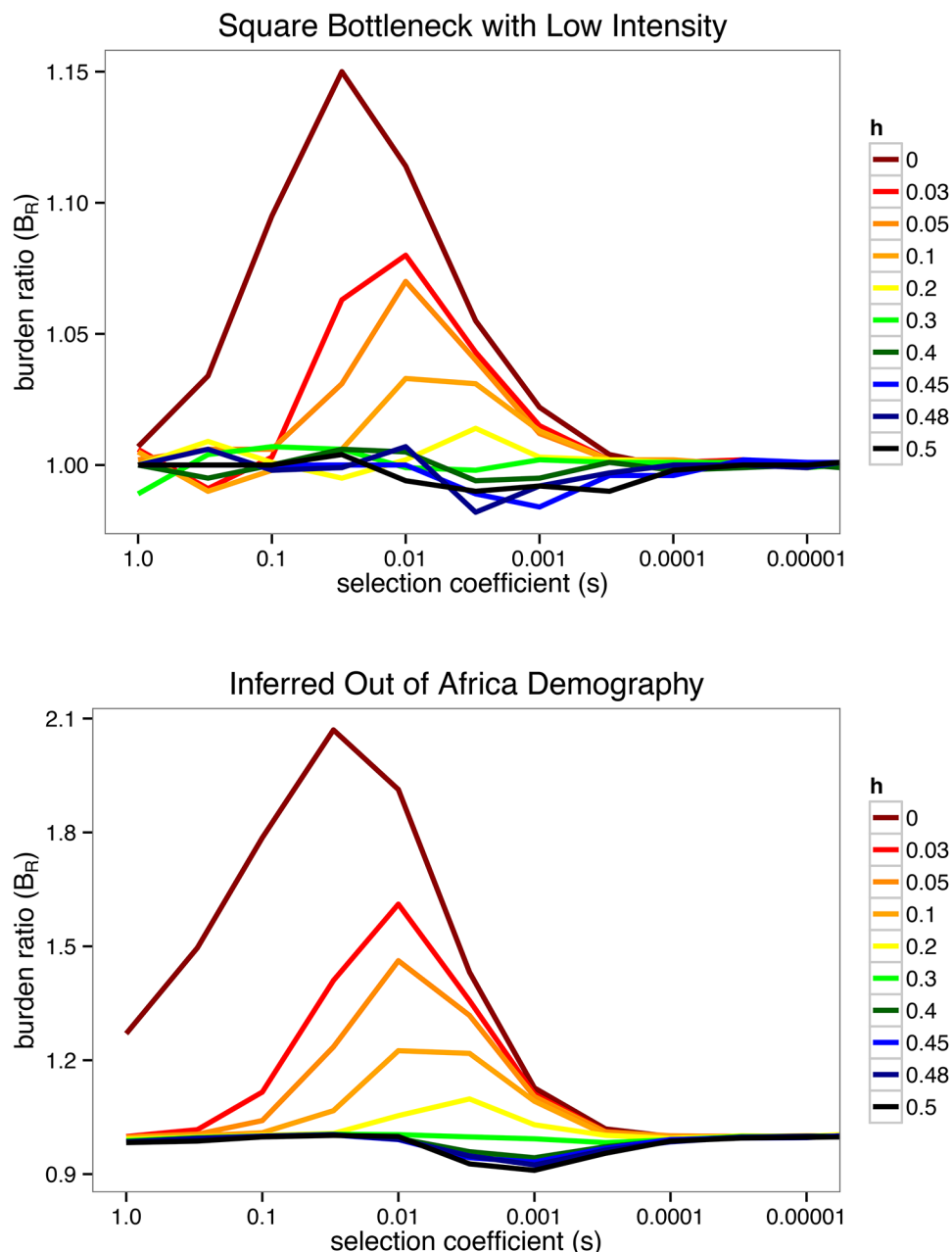
Fig 3. The B_R statistic at the time of observation. ABOVE: At the time of observation t_{obs} , the value of B_R(t_{obs}) is plotted as a function of the average strength of selection s and dominance coefficient h . Dominance coefficients appear as solid lines with fully recessive selection ( h = 0 ) at the top and purely additive selection ( h = \frac{1}{2} ) at the bottom. For strong selection B_R \rightarrow 1 due to the rapid transient response. For weak selection B_R \rightarrow 1 due to the nearly neutral insensitivity to the bottleneck. For some intermediate dominance coefficient h_c , a critical value occurs ( h_c \sim 0.25 in the example shown, but explored more generally in S1 Text ) where additive and recessive effects cancel, yielding B_R(h_c) \sim 1 . A low intensity bottleneck ( I_B = 0.05 ) is shown, with parameters 2N_0 = 20000 , 2N_B = 2000 , T_B = 100 , and t_{obs} = 1000 . BELOW: The same range of parameters is plotted for a realistic demographic model of the Out of Africa event comparing Africans and Europeans [48], where B_R = \langle x \rangle_{African} / \langle x \rangle_{European} . The European bottleneck has estimated intensity I_B \sim \mathcal{O}(0.5) , an order of magnitude stronger than the simple bottleneck above, allowing for potentially observable deviations from B_R \sim 1 if a large fraction of analyzed variants act recessively with h < h_c \sim 0.25 .
