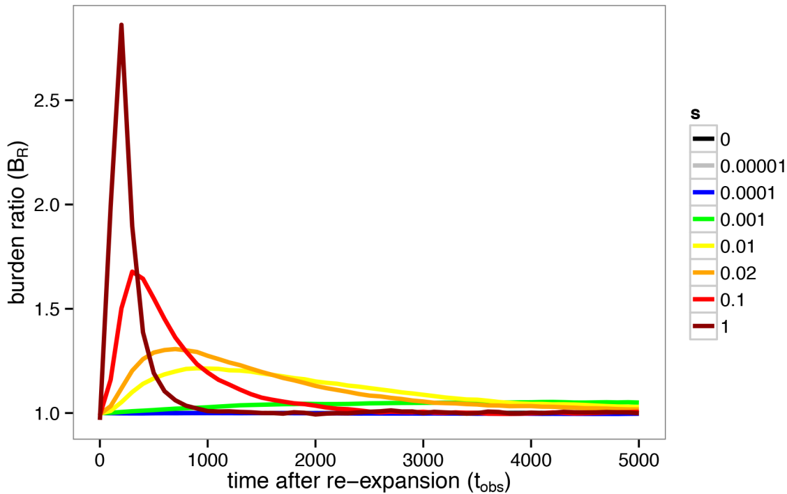
Fig 2. Time dependence of the B_R statistic after re-expansion. The time dependence of B_R(t) after a population bottleneck is shown for alleles under recessive selection ( h = 0 ) for various selection strengths. Peak B_R values vary in both magnitude and time as a function of s . The founded population was simulated with 2N_0 = 20000 , 2N_B = 2000 , and T_B = 200 and plotted for 5000 generations after re-expansion.
