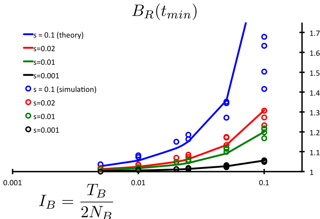
Fig 4. Comparisons of analytic and simulation results. Maximum response values of the burden ratio B_R(t_{min}) are plotted for recessive selection as a function of bottleneck intensity. A wide range of parameter sets is plotted with all combinations of 2N_B = \{2000, 1000, 400, 200, 100\} , s = \{0.1, 0.02, 0.01, 0.001\} , T_B = \{200, 100, 50, 20, 10\} , each simulated for 10^8 nucleotide sites. For relatively low intensity bottlenecks we note excellent agreement over the parameter ranges plotted. Intensities with I_B = T_B/2N_B > 0.1 are excluded, as the single-generation bottleneck scaling breaks down in favor of a long bottleneck scaling. The approximation necessarily weakens for simulations that represent longer bottlenecks, and only for strong selective coefficients, as expected. This quantifies the limitations of the single-generation bottleneck approximation, as we observe substantial deviation only around I_B = 0.1 and with selection strength s = 0.1 .
