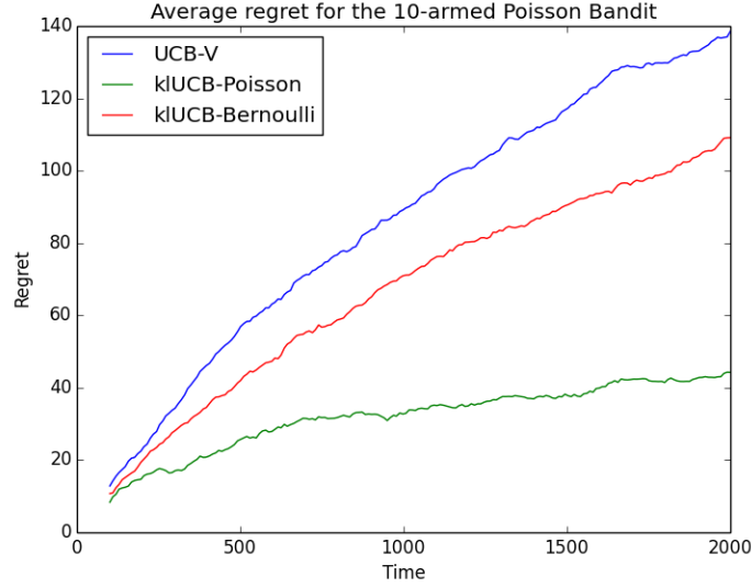
Figure 4: 10-armed Poisson Bandit Algorithm Performance
