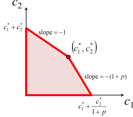
Figure B2: A two-part budget set. Such budget sets consist of: (i) a budget curve that has slopes of -1 and -(1+p) to the left and right of a kink at (c_1^*, c_2^*) ; and (ii) none, some or all of the points of the ambient budget set that lie below or to the left of the budget curve.
