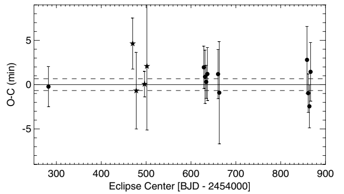
Figure 9. Observed minus calculated secondary eclipse times using the best-fit period from the transit fits and allowing the phase of the secondary eclipse to vary freely. Filled circles are eclipse times reported in this paper, and filled stars are additional 3.6 and 4.5\mu\text{m} eclipse times from Stevenson et al. (2010). The solid line indicates the best-fit phase, with \pm 1\sigma uncertainties plotted as dashed lines.
