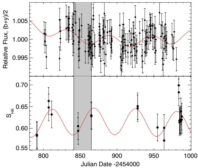
Figure 11. Upper panel plots APT measurements of variation in the averaged Strömgren b+y band fluxes (filled circles) obtained for GJ 436 between UT 2008 November 30 and UT 2009 May 29, where the epoch of our 2009 Spitzer observations is denoted by the gray shaded region. These bandpasses are sensitive to the rotation-modulated flux of the star, which we find has a best-fit period of 57 days during this epoch. We overplot a red curve showing our best sine-curve fit for the spot modulation, together with a quadratic function of time to describe the evolution of the spot coverage on longer timescales. The lower panel shows the measured S_{\text{HK}} values for GJ 436 from the Keck HIRES instrument during this same period (Isaacson & Fischer 2010), with a best-fit sine + quadratic function overplotted in red. Error bars for both panels are set equal to the standard deviation of the residuals. Although the best-fit period of 57 days for the S_{\text{HK}} data during this epoch is only marginally significant, the S_{\text{HK}} values appear to be anti-correlated with the flux variations. This is consistent with a model in which increased magnetic activity is associated with the presence of spots or other dark regions on the surface of the star.
